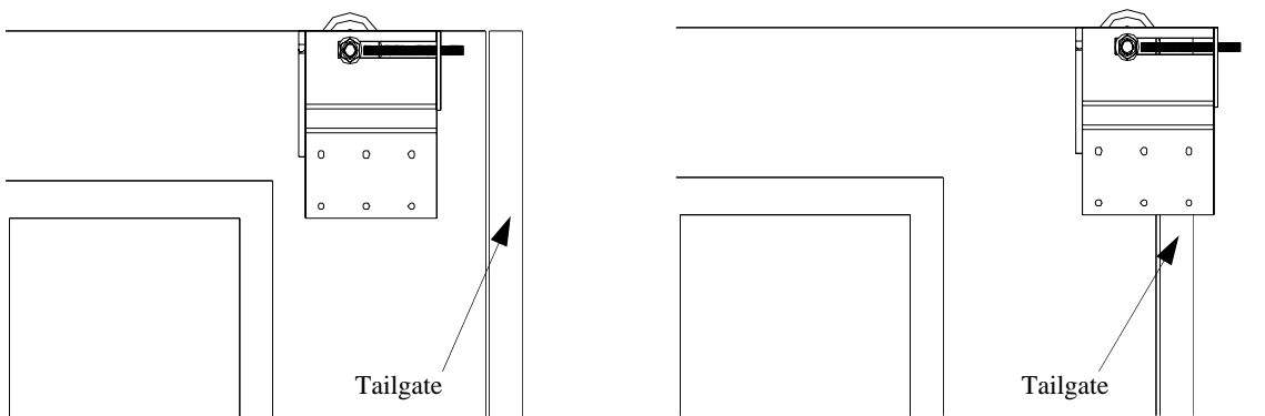
Swing style tailgate: Idler assembly is moved forward to prevent interference with the opening process.
